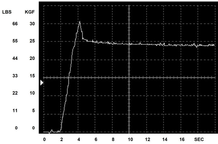
LOCK OUT; NYLON 1,8 / 4,2 % / 20 KGF. TENSION LOSS = 8 KGF (17,6 LBS)
