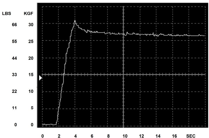
LOCK OUT; NYLON 1,6 / 3,4 % / 20 KGF. TENSION LOSS = 5 KGF (11 LBS)
