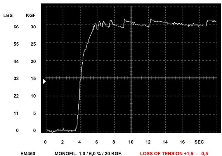
HIGH END ELECTRONIC TENSIONER
