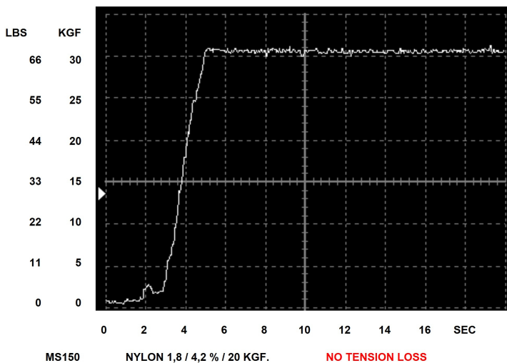
"SMART-SPRING TENSIONER"
